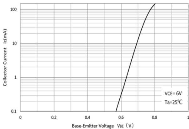
Fig 5: Base-Emittor Voltage
