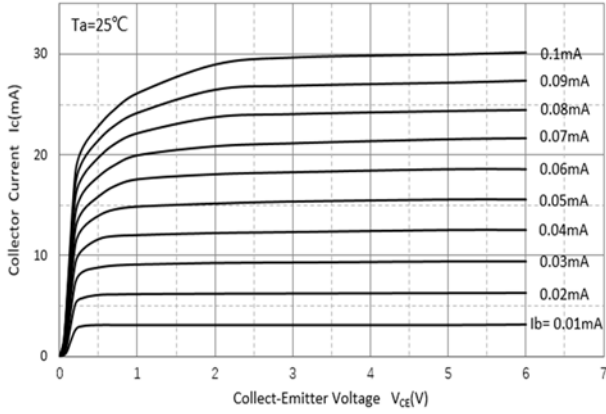
Fig 1: Static Characteristics
