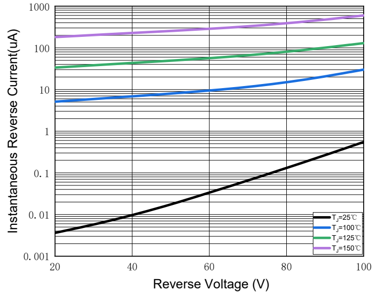
Fig.4: Typical Reverse Leakage Characteristics(Per Diode)
