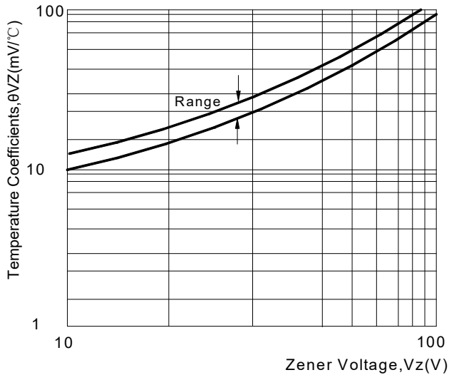
FIG3: Temperature Coefficients v.s. Zener Voltage
