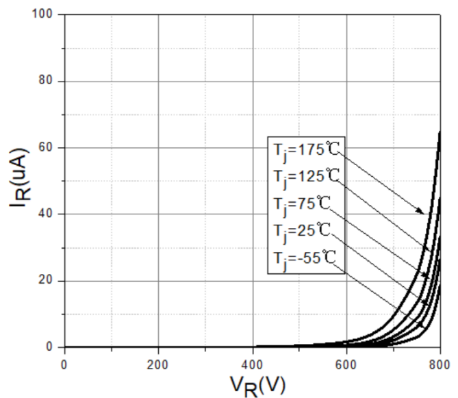
Figure 2. Reverse Characteristic
