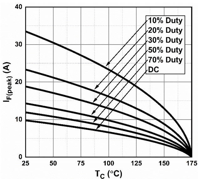
Figure 7. Current Derating
