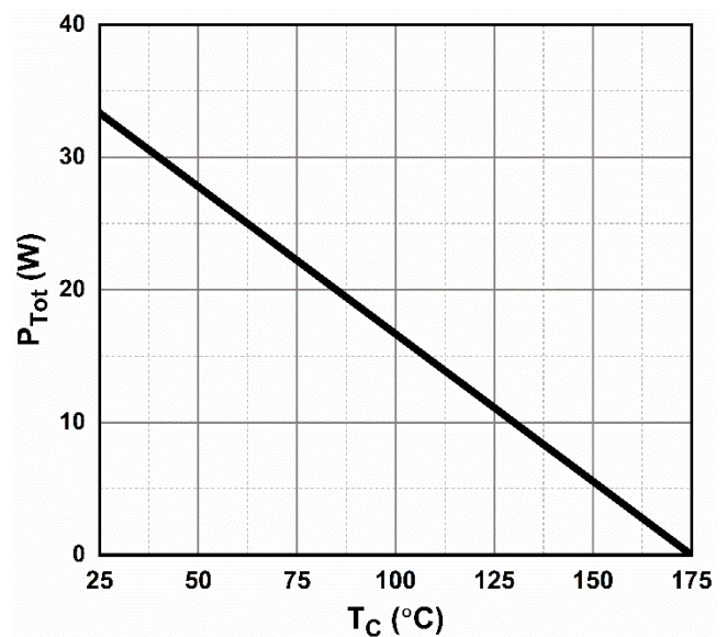
Figure 6. Power Derating
