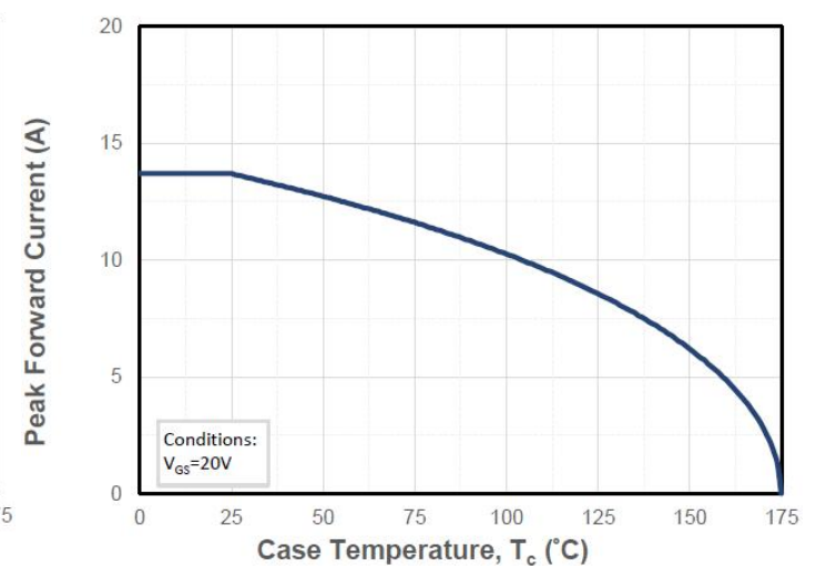
Figure 14. Drain Current Derating vs. Case Temperature
