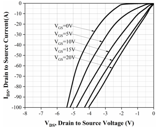
Figure 10. 3 rd quadrant characteristic at T_j = 25^\circ\text{C}
