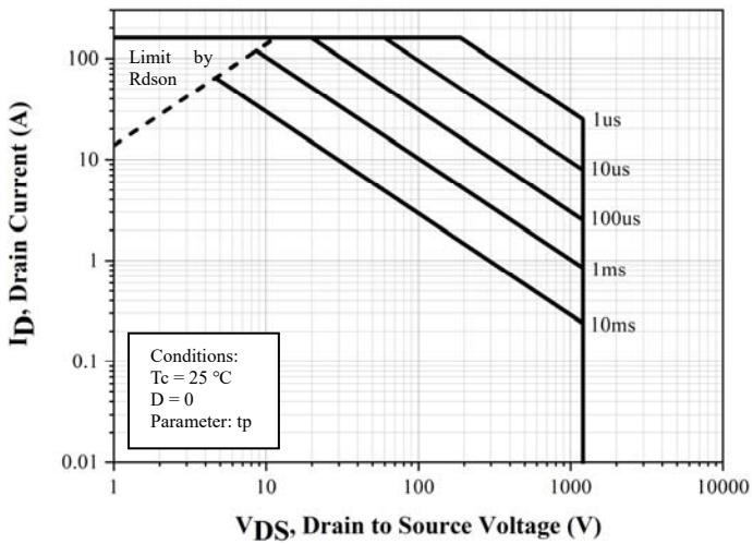
Figure 23. Drain to Source Voltage (V)
