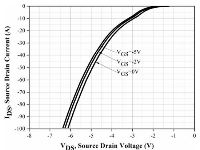
Figure 8. Body diode characteristic at Tj = 25 °C
