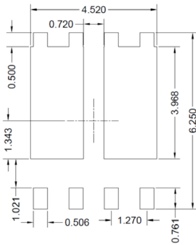
Suggested Solder Pad Layout Top View
